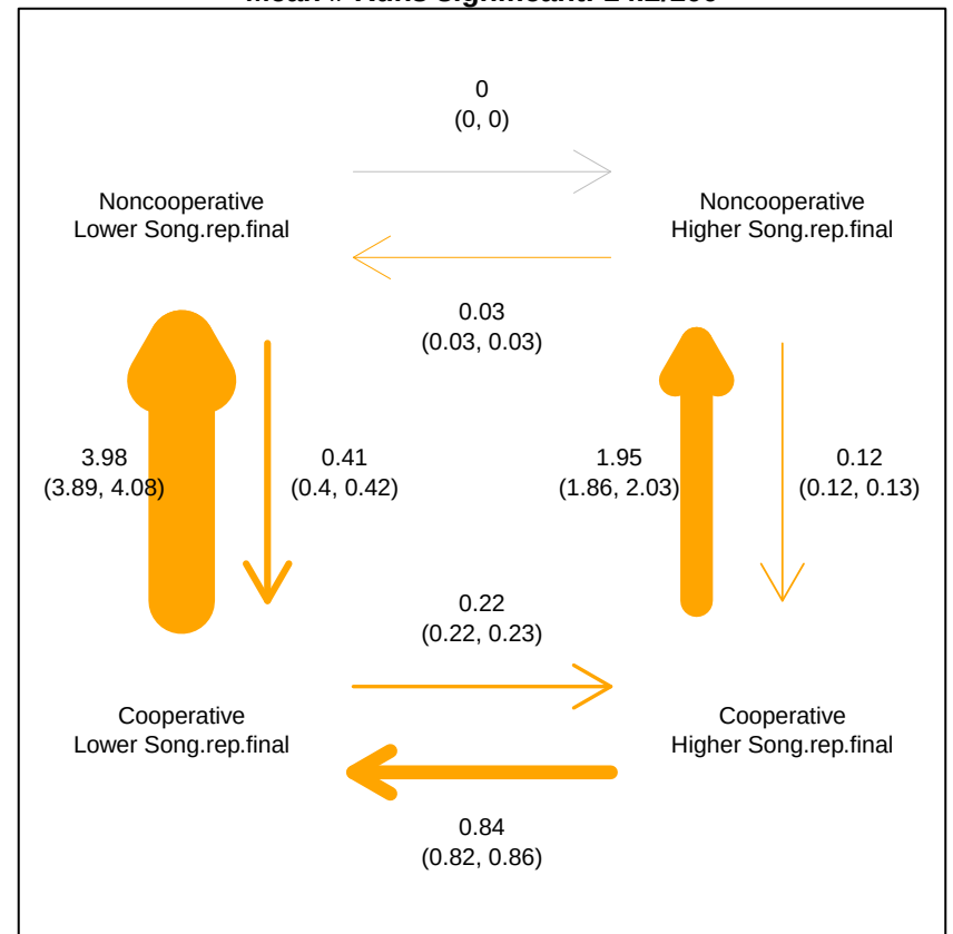
Thresholds \geq 8.5 - < 34 (24) Mean # Runs significant: 14.2/100
